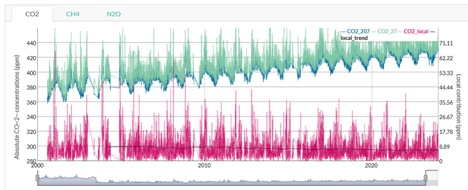
Measured concentrations at Cabauw
